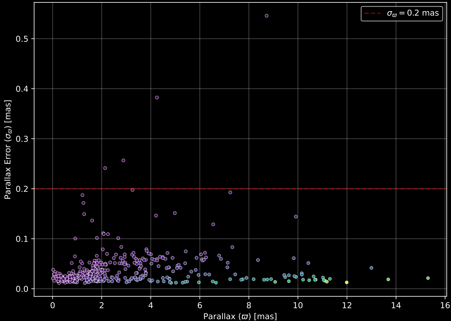
APOGEE DR17 Field: [060+75] Parallax Quality (n= 406)
