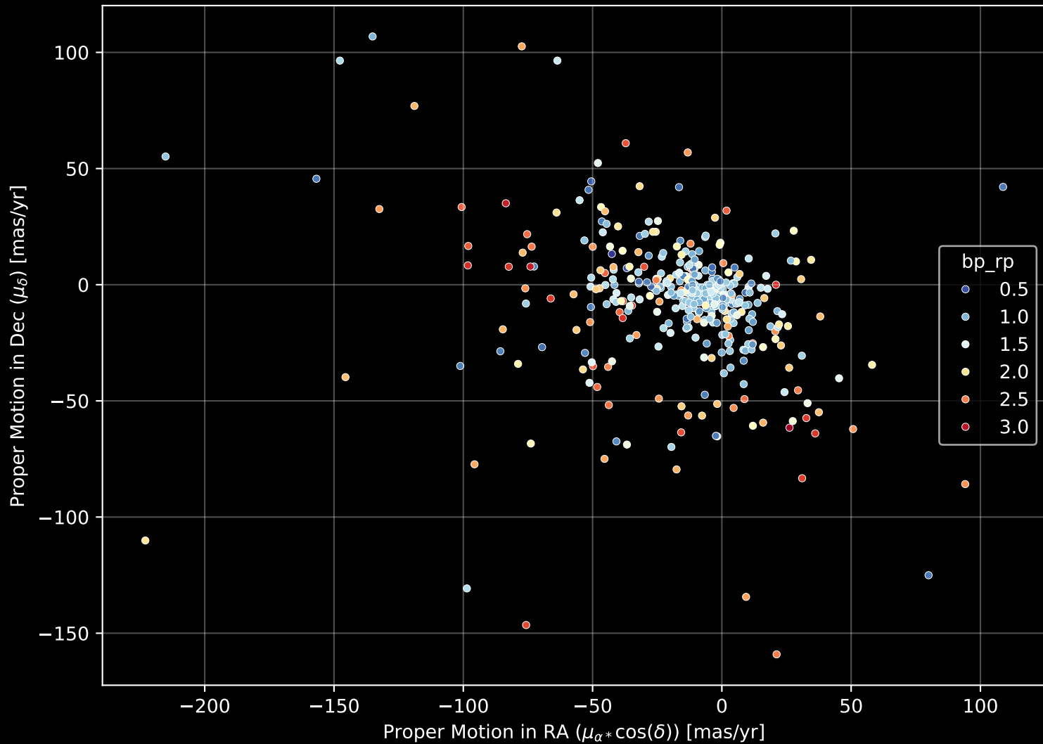
APOGEE DR17 Field: [060+75] Proper Motion Diagram (n= 406)
