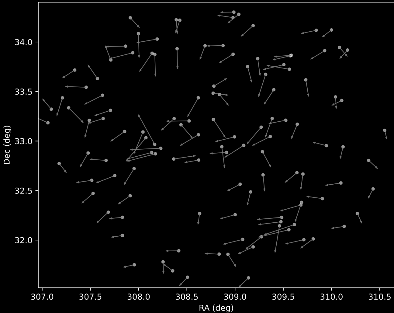
APOGEE DR17 Cluster 14 Proper Motion Vectors (n=120)
