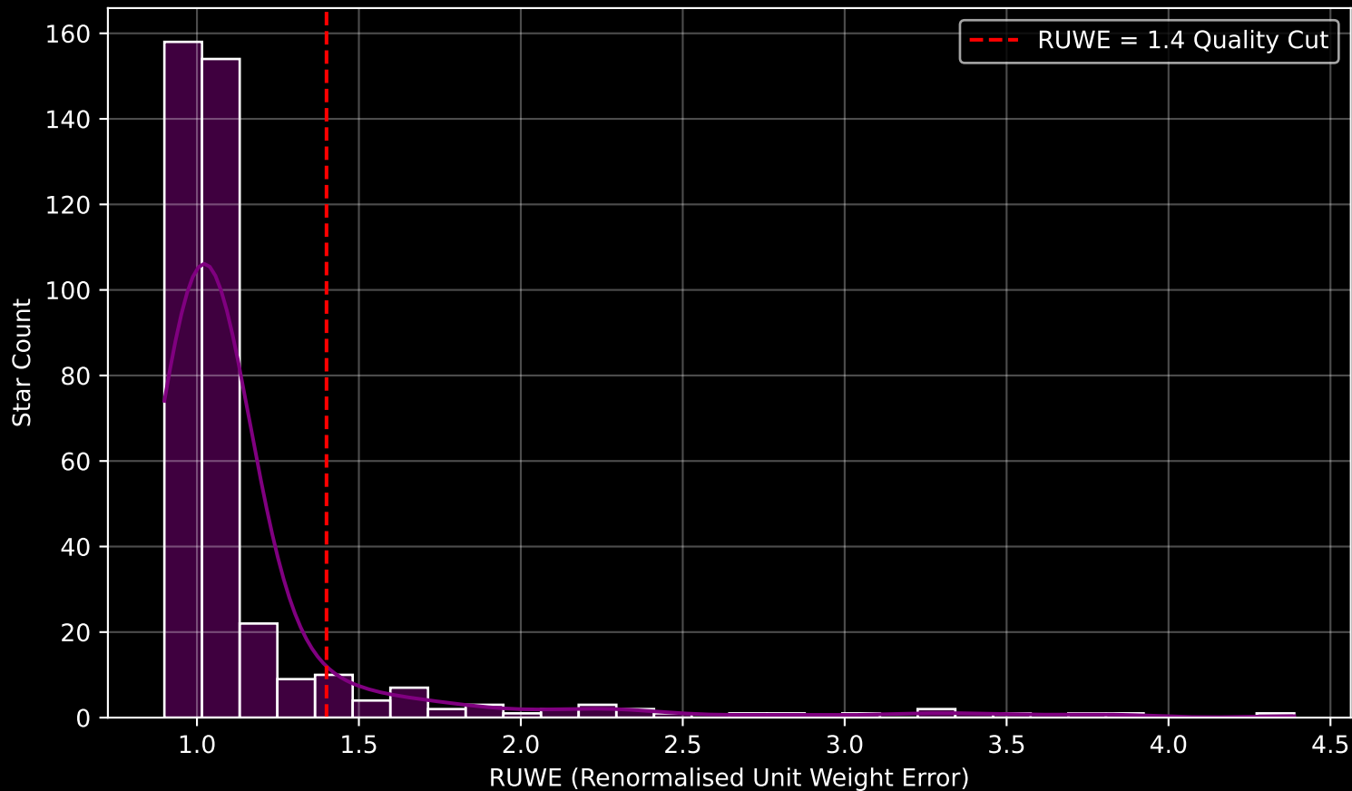
GAPOGEE DR17 Field [060+75] RUWE Distribution (n= 388)
