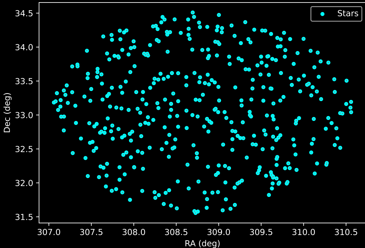
APOGEE DR17 Field: [060+75] Proper Motion Vectors for Gaia Star Field (n= 406)
