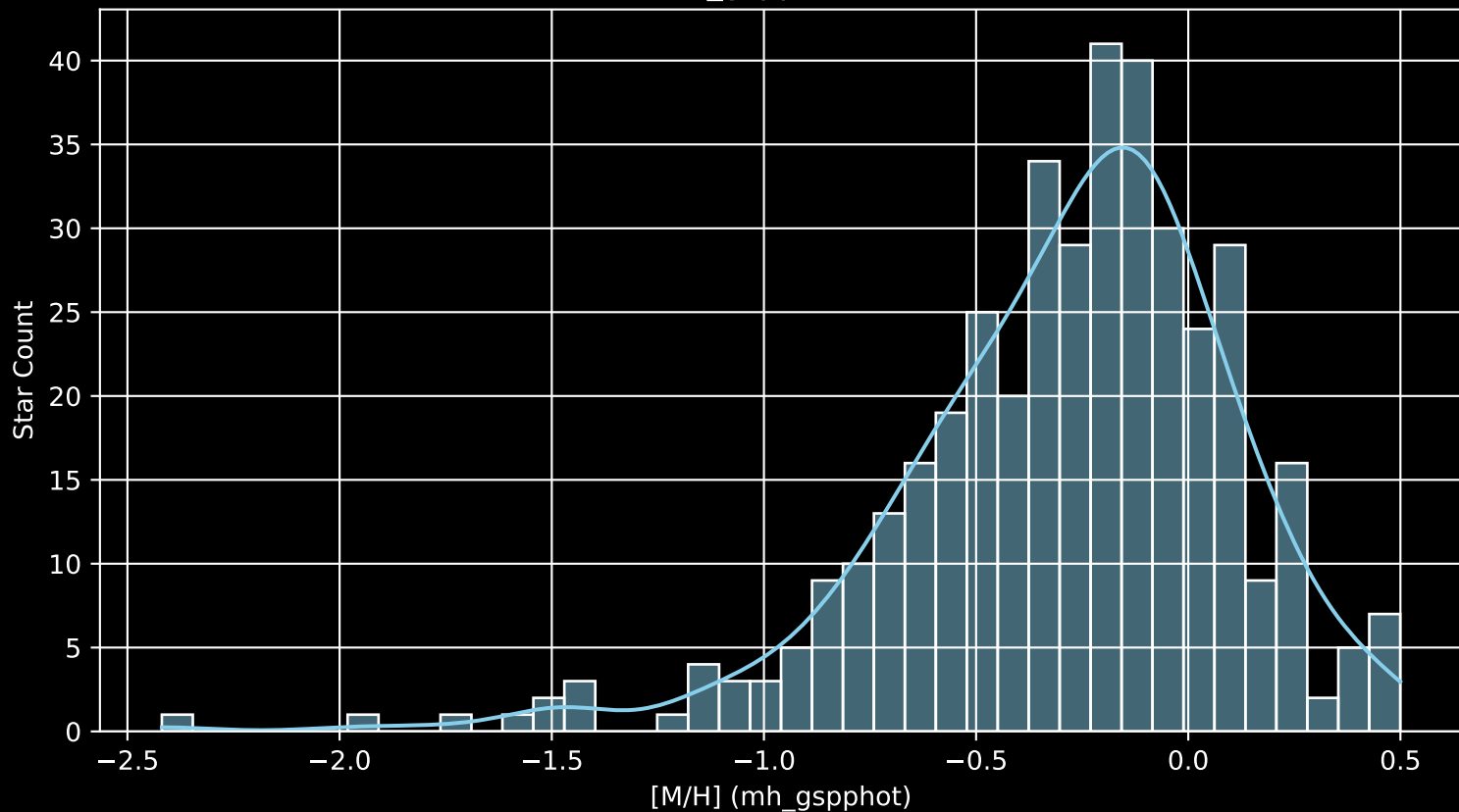
APOGEE DR17 Field: [060+75 [M/H] (mh_gspphot) (n= 403)
